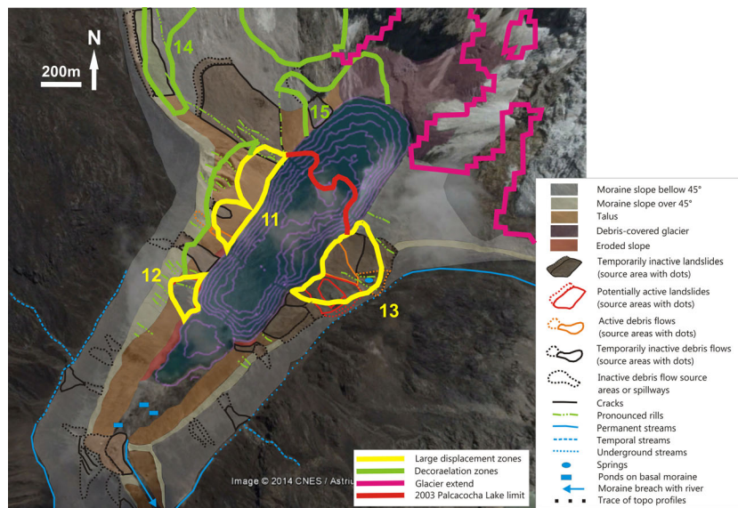
Fig. 9 Results of the DInSAR analysis interpretation (for additional information, see Online Resource 1). Yellow outlines define zones with detected movement rates of 10\text{--}50\text{ cm year}^{-1} with years when the major displacements were detected. Areas on the orographic right slopes of the Palcacocha Lake were detected with ALOS PALSAR image pairs with a time interval of 46 days and ENVISAT ASAR image pairs with a time interval of 35 days. The area on the left moraine slope was identified using ERS SAR image pairs with 35-day interval. Areas with decorrelation observed in yearly or monthly DInSAR interferograms are shown by green lines . The signal decorrelation could be caused by snow patches near the glacier or by large mobility of superficial material or landslide activity. Extent of the Palcacocha Lake in 2003 is shown by red outline . Glacier extents from Randolph Glacier Inventory Version 4.0 (Arendt et al. 2014) are shown by pink lines . Background image is August 2013 Google Earth satellite image
