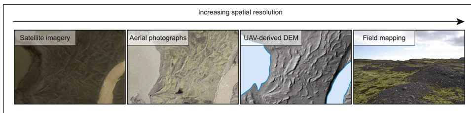
Fig. 17. Geomorphological mapping of the foreland of Skálafellsjökull, an active temperate outlet of Vatnajökull, SE Iceland. (A) Digital aerial photographs (2006; 0.41 m GSD; Loftmyndir ehf ), pan-sharpened WorldView-2 multi-spectral satellite imagery (2012; 0.5 m GSD; European Space Imaging ), a UAV-derived DEM (2013; 0.09 m GSD) and field mapping were employed to produce the mapping extract (B). A compromise on the level of detail was made, with annual moraines mapped along crestlines due to image resolution and map readability. This mapping detail was sufficient for calculating crest-to-crest moraine spacing (ice-margin retreat rates) shown in (C), which was the principal purpose of the study. Modified from Chandler et al. (2016a, b).
