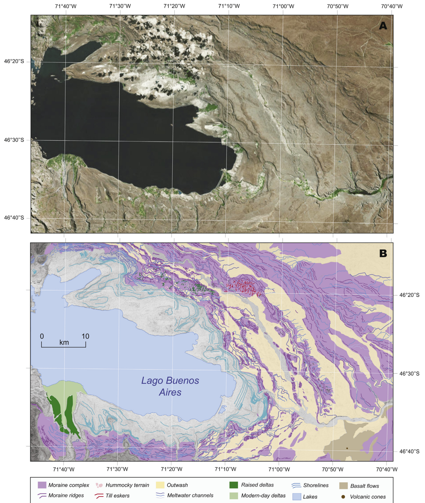
Fig. 3. Example of geomorphological mapping produced through on-screen vectorisation (tracing) in GIS software. Satellite image (A) and geomorphological mapping (B) showing suites of moraines formed by the Lago General Carrera–Buenos Aires ice lobe of the former Patagonian Ice Sheet, located to the east of the present-day Northern Patagonian Icefield. A combination of remotely-sensed datasets and field mapping were used to circumvent issues of localised cloud cover, as visible in (A). Where areas were obscured, SPOT-5 and DigitalGlobe images available in Google Earth were used. The geomorphological map extract is taken from Bendle et al. (2017a).
