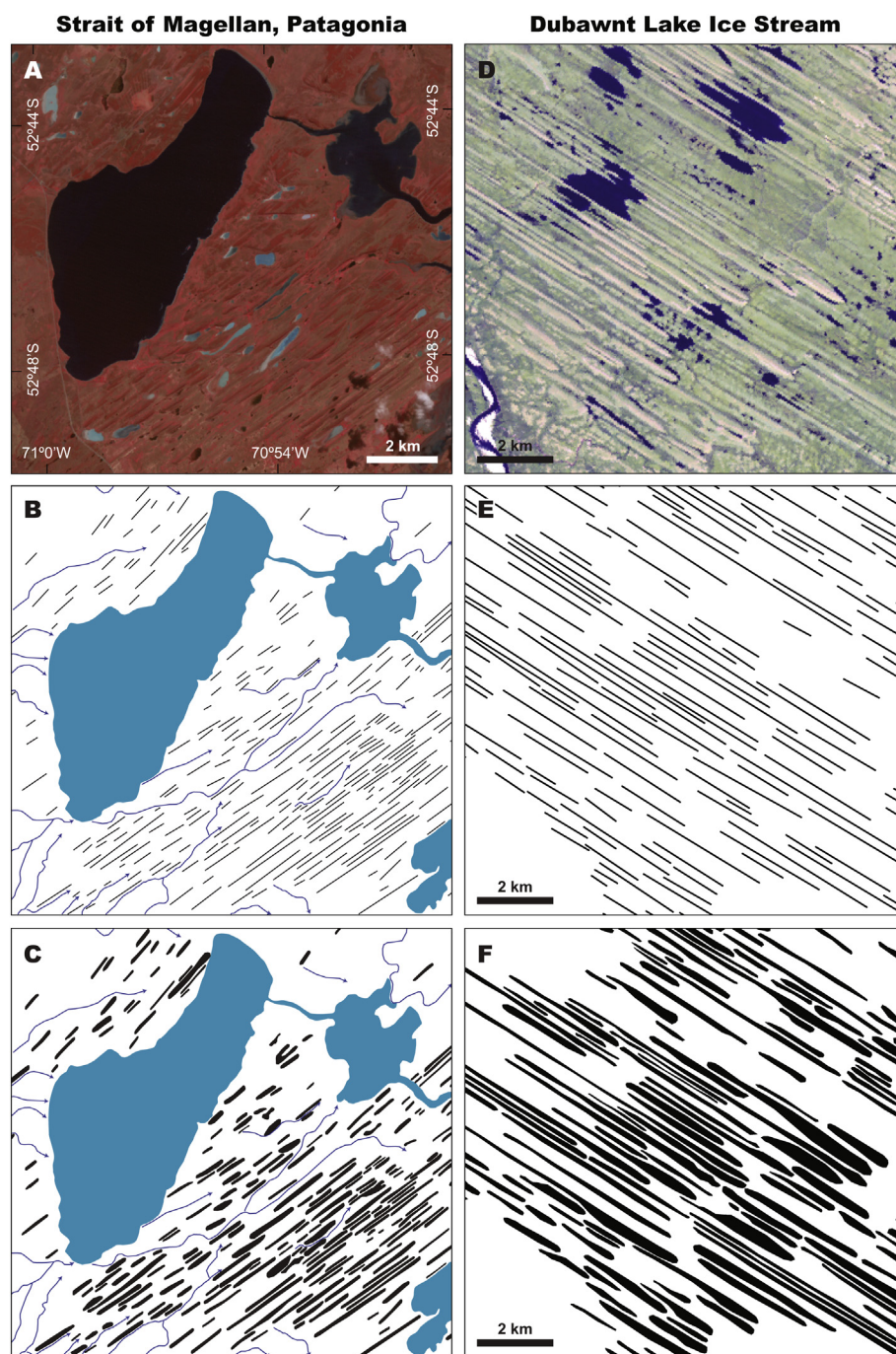
Fig. 13. Example mapping of subglacial bedforms from the Strait of Magellan, Patagonia (A–C), and the Dubawnt Lake Ice Stream (D–F). The bedforms are mapped as polylines along landform crests in (B) and (E), and they are mapped as polygons delineating lower-break-of-slope in (C) and (F). The Dubawnt Lake Ice Stream polylines (Stokes and Clark, 2003) and polygons (Dunstone, 2014) were mapped by different mappers at different times, which may account for small inconsistencies. For further details on the bedform examples from the Strait of Magellan, see Lovell et al. (2011) and Darvill et al. (2014).
