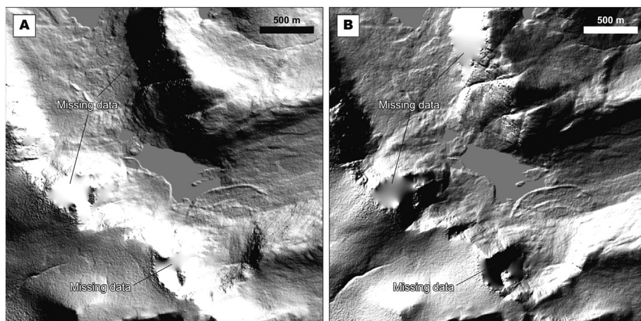
Fig. 12. Extracts from hillshaded relief models of Ben More Coigach, NW Scottish Highlands, showing the effect of geometric artefacts on the models. The hillshades were generated with azimuths of 45° (A) and 315° (B). Stretching of upland terrain during processing of the DEM data results in blurred regions on the hillshaded relief models. NEXTMap DSM from Intermap Technologies Inc. provided by NERC via the NERC Earth Observation Data Centre.
