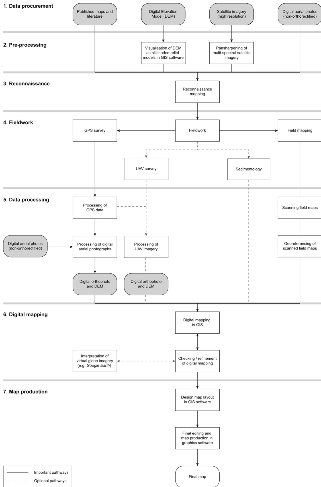
Fig. 19. Idealised workflow for mapping alpine- and plateau-style ice mass geomorphological imprints. In this scenario, digital remotely-sensed datasets are used and this necessitates image processing before mapping is undertaken. Ideally, GNSS surveys would be conducted in order to process digital aerial photographs, as depicted in the workflow. Some pathways are optional (grey dashed lines) depending on data availability and the feasibility and applicability of particular methods. Although sedimentology is shown as ‘optional’, it is highly desirable to undertake sedimentological investigations, wherever possible. Alternative image processing solutions are available and readers should consult with the detailed processing workflow which is available as Supplementary Material.
