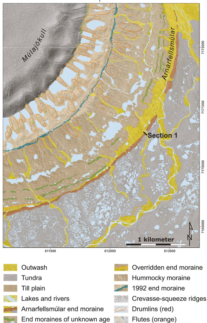
Fig. 16. Geomorphological mapping (A) from the Múlajökull foreland, Iceland, completed as part of a process-oriented study examining the internal architecture and structural evolution of a Little Ice Age terminal moraine at this surge-type glacier (Benediktsson et al., 2015). The mapping was combined with sedimentological investigations (B) to produce a process-form model of moraine formation and evolution (C).
