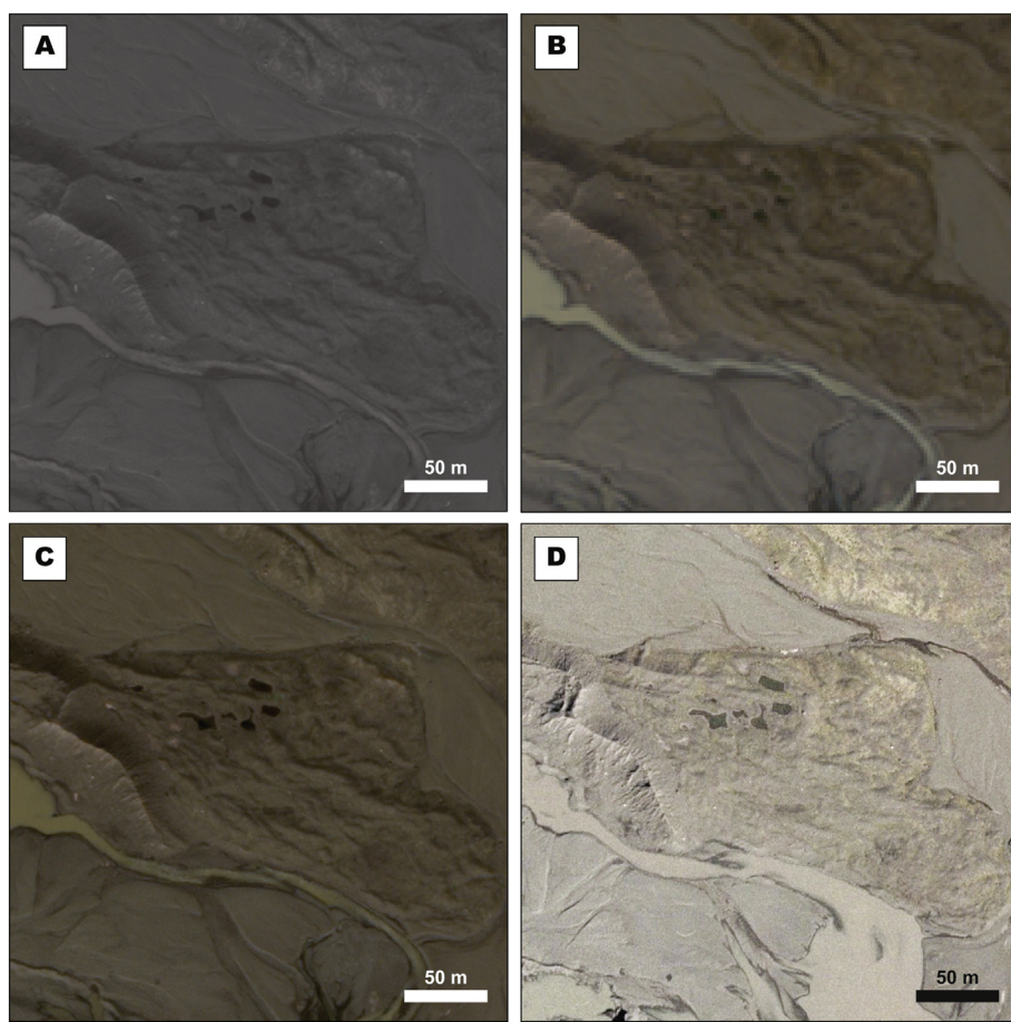
Fig. 4. Comparison of WorldView-2 satellite imagery (June 2012, European Space Imaging) with digital colour aerial photographs (2006, Loftmyndir ehf) for the Skálafellsjökull foreland, SE Iceland. (A) Panchromatic satellite image (0.5 m ground sampled distance, GSD). (B) Multispectral satellite image (2.0 m GSD). (C) Pansharpened three-band natural colour satellite image (0.5 m GSD). (D) Digital colour aerial photographs (0.41 m GSD). The satellite imagery is of sufficient resolution to allow mapping of small-scale (< 2 m in height) annual moraines (see Chandler et al., 2016a, b).
