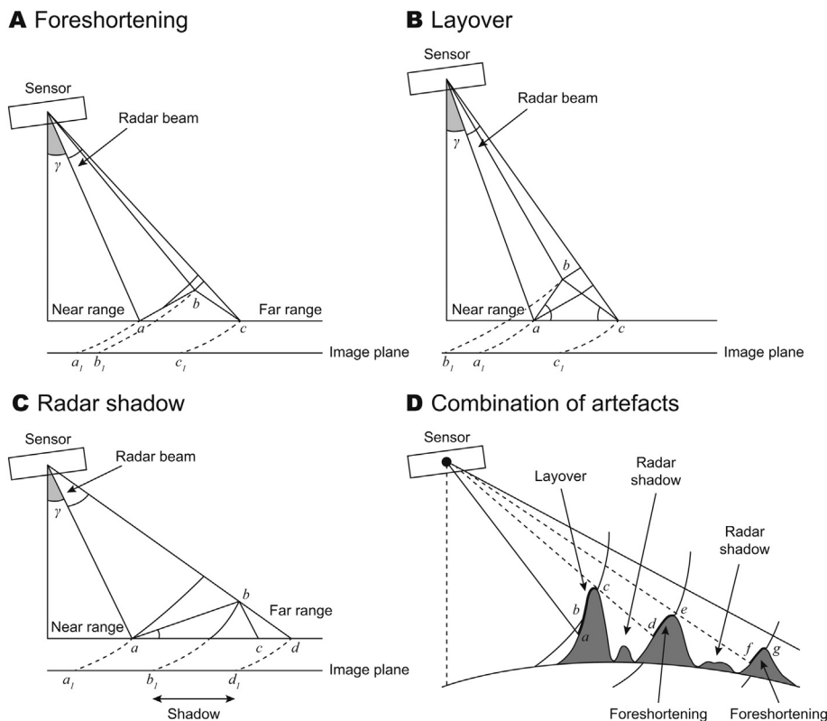
Fig. 11. Geometric artefacts that may be present in space- and air-borne radar captured imagery, resulting from the effects of relief. (A) Foreshortening, occurring where the slope of the local terrain is less than the incidence angle ( \gamma ). The facing slope, a - b , becomes compressed to a_1 - b_1 in the resulting image. (B) Layover, occurring in steep terrain when the slope angle is greater than the incidence angle. As a mountain-top, b , is closer to the sensor than the base, a , this causes layover in the imagery (an incorrect positioning of b_1 relative to a_1 ). (C) Radar shadow in areas of rugged terrain as the illumination is from an oblique source. No data is recorded for the region b_1 - d_1 . (D) In regions of varying topography, a combination of artefacts may be present: points b and c will be impacted by layover and will be positioned incorrectly relative to a ; no data will be recorded for the region between c and d due to radar shadow; foreshortening occurs at slope facet d - e ; further radar shadow occurs at e - f ; and foreshortening at f and g . After Clark (1997).
