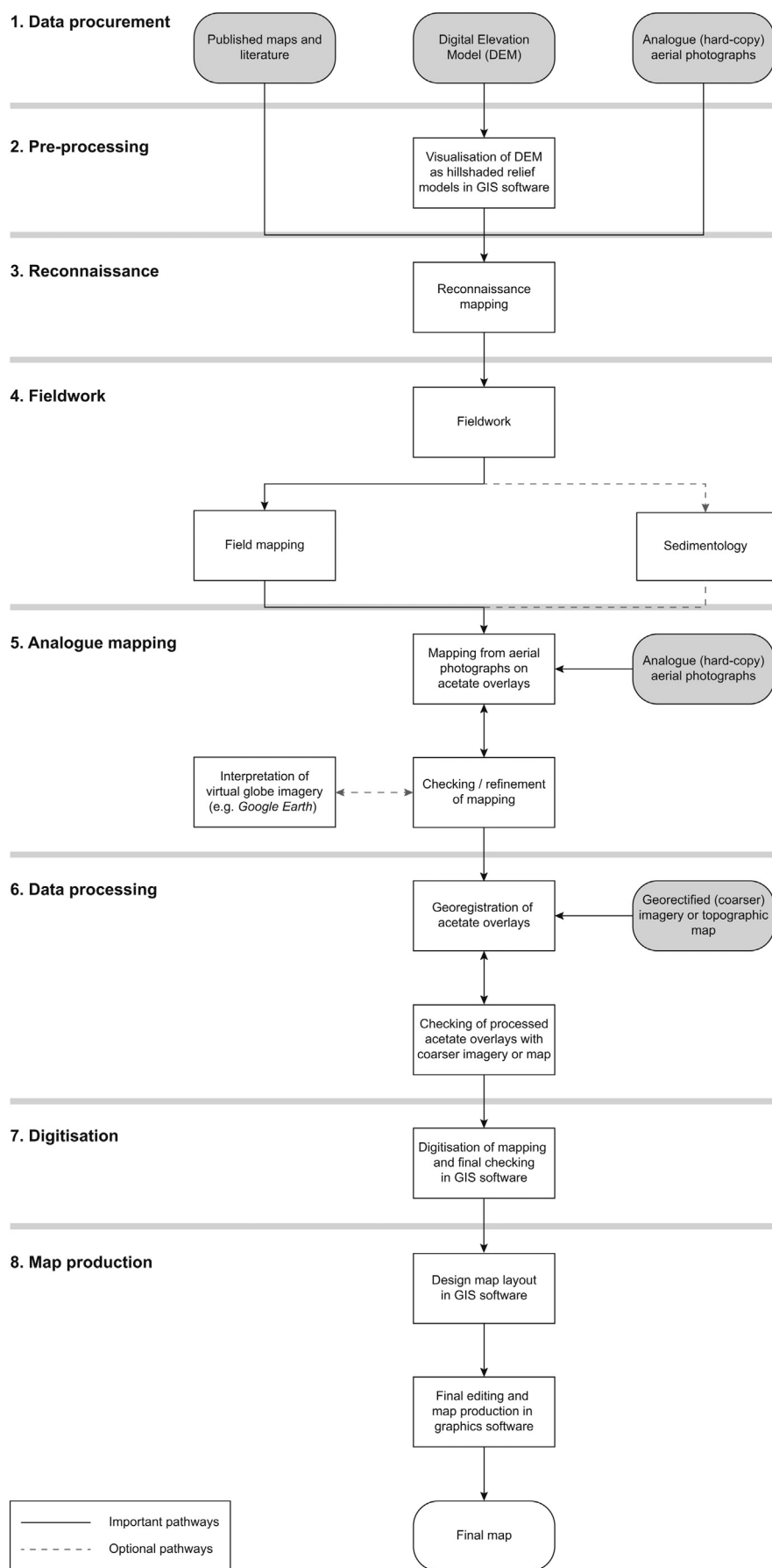
Fig. 20. Idealised workflow for mapping alpine- and plateau-style ice mass geomorphological imprints. In this scenario, analogue (hard-copy) aerial photographs are used and this necessitates image processing after mapping is undertaken. Some pathways are optional (grey dashed lines) depending on data availability and the feasibility and applicability of particular methods. Although sedimentology is shown as ‘optional’, it is highly desirable to undertake sedimentological investigations, wherever possible. Alternative image processing solutions are available and readers should consult with the detailed processing workflow which is available as Supplementary material.
