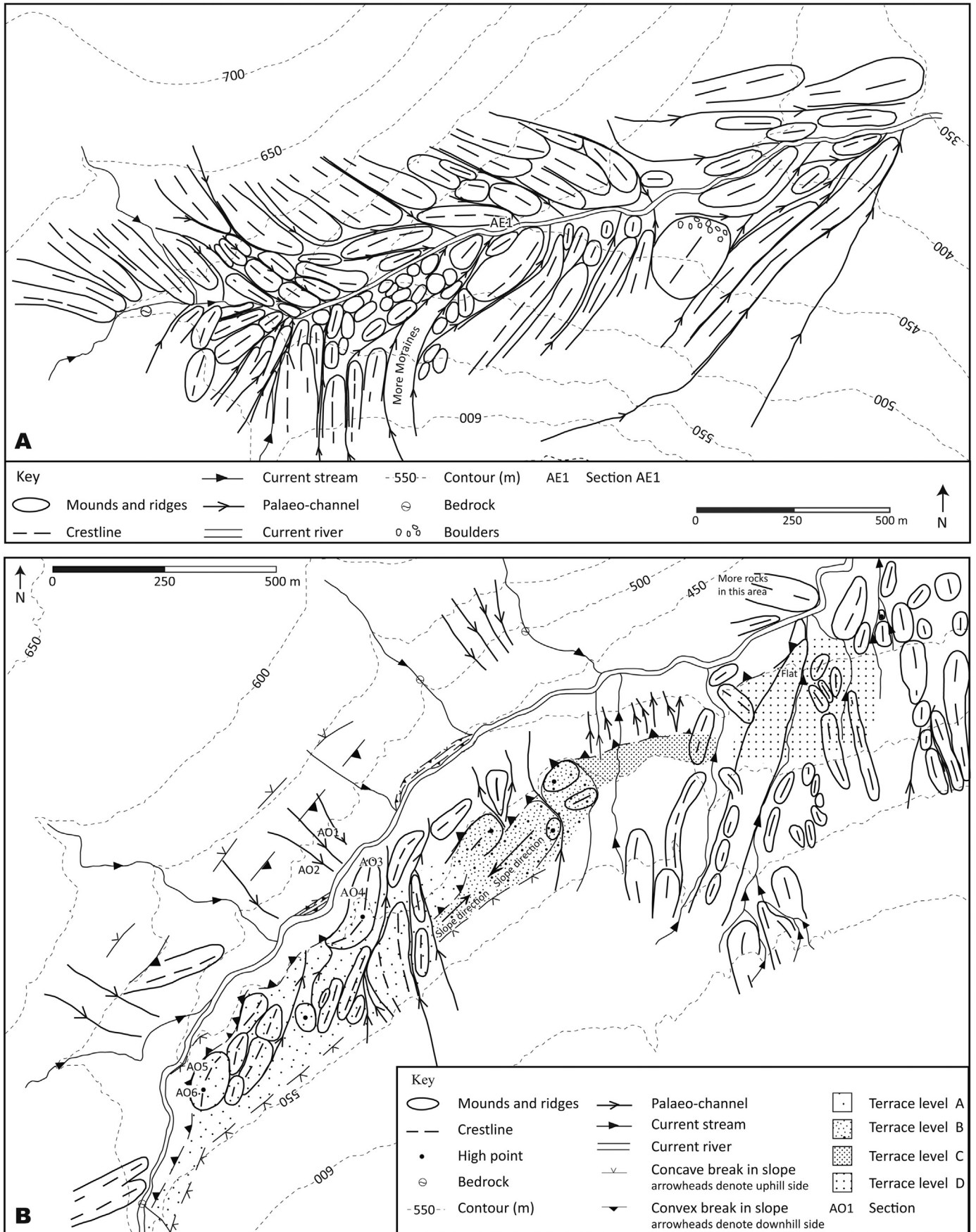
Fig. 1. Vectorised versions of two geomorphological maps drawn in the field for (A) Coire Easgairn and (B) Glen Odhar in the Monadhliath, Central Scottish Highlands. These field maps were used in the production of a 1: 57,500 geomorphological map for the entire region (Boston, 2012a, b).
