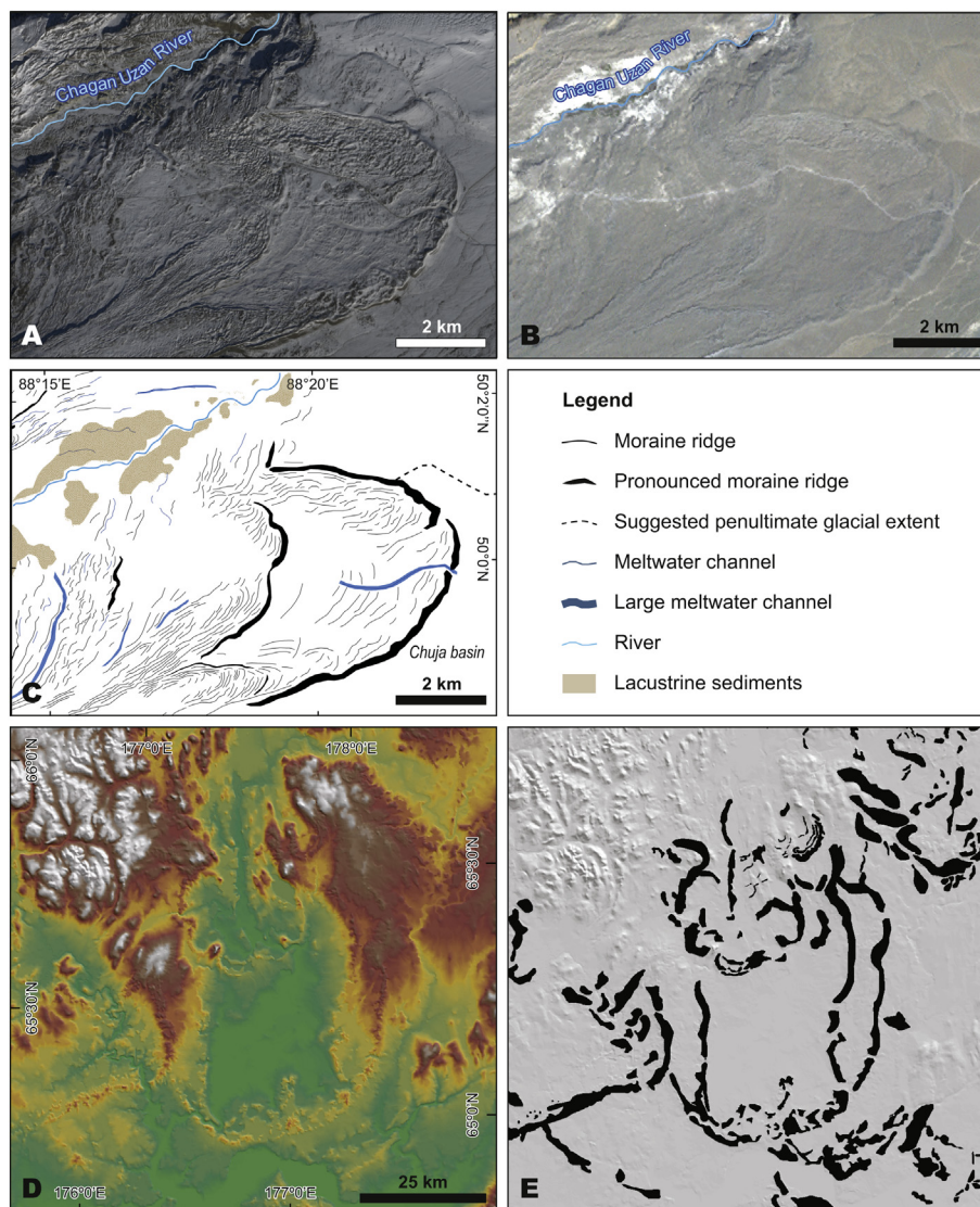
Fig. 15. Examples of landforms in icefield and valley glacier settings mapped on medium to coarse resolution imagery. Landforms observed in the Chagan Uzun Valley, Russian Altai, displayed on (A) SPOT image and (B) Landsat 7 ETM+ image. (C) Associated geomorphological map extract from Gribenski et al. (2016). Moraines in the Anadyr Lowlands, Far NE Russia, displayed on (D) semi-transparent shaded ViewFinder Panorama (VFP) DEM data (NE solar azimuth) draped over the raw VFP DEM. (E) Associated mapping of moraines (black polygons) from Barr and Clark (2012).
