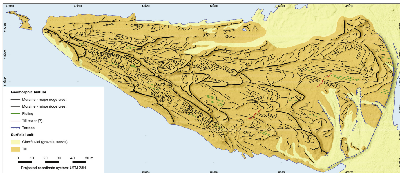
Fig. 7. High-resolution geomorphological mapping of part of the Fláajökull foreland, Iceland, based on UAV-derived imagery (Evans et al., 2016a). A 1: 350 scale version of this map is freely available for download from Journal of Maps : https://doi.org/10.1080/17445647.2015.1073185 .
