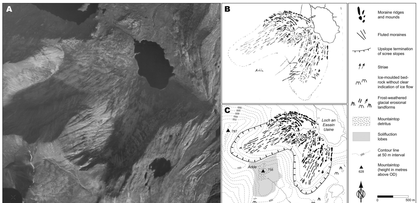
Fig. 2. The aerial photograph overlay-mapping process using an example from the mountain Arkle, NW Scotland. (A) aerial photograph at an average scale of \sim 1:25,000 (extract from photo 38 88 087; ©RCAHMS 1988); (B) scan of original overlay mapped through a stereoscope from (A) (see Section 3.1.2 for method description), focusing on moraines, fluted moraines and the approximate upper limit of scree slopes as seen from the aerial photograph; (C) compiled, rectified geomorphological map, incorporating moraines and fluted moraines from (B) and additional data from field mapping, such as the exact upper limits of scree slopes, orientation of striae, solifluction lobes and mountaintop detritus. For description and interpretation of the geomorphology, see Lukas (2006).
