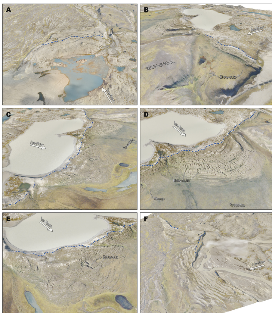
Fig. 6. Views at various points along the length of the 1890 surge end moraine at Eyjabakkajökull, Iceland, visualised in 3D within ESRI ArcScene (Benediktsson et al., 2010). Aerial orthophotographs from 2008 are draped over a 3 m grid DEM with 1.5x vertical exaggeration. For reference to the individual image panels, readers are directed to the original publication.
