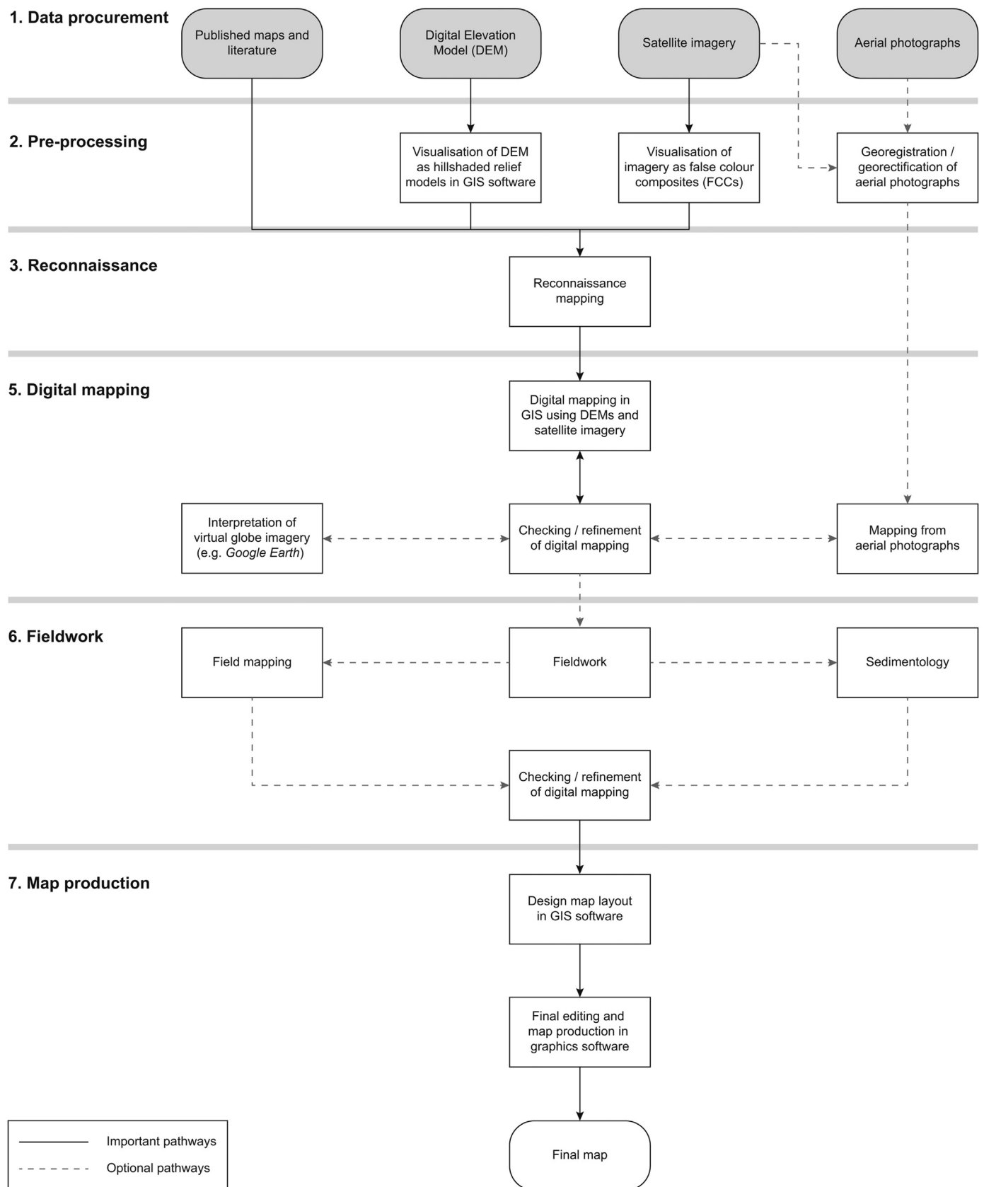
Fig. 18. Idealised workflow for mapping palaeo-ice sheet geomorphological imprints. Some pathways in the workflow are optional (grey dashed lines) depending on data availability and the feasibility and applicability of particular methods. Note, where analogue (hard-copy) aerial photographs are used for mapping, processing of acetate overlays would be undertaken after mapping from the aerial photographs. Further details on image processing are shown on the processing workflow available as Supplementary Material.
