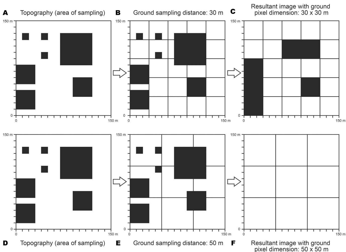
Fig. 10. Conceptual diagrams illustrating the distinction between Ground Sampled Distance (B and E) and pixel size (C and F). The ground distances between two measurements by the detector (i.e. the Ground Sampled Distances) are 30 m and 50 m in (B) and (E), respectively. These Ground Sample Distances are then assigned to pixels in the resulting 30 x 30 m (C) and 50 x 50 m (F) digital images. Note, resultant images may fail to accurately represent the shape of the objects (upper row) or may even fail to reproduce them (lower row), even where the size of the object is the same or larger than the sampling distance.
