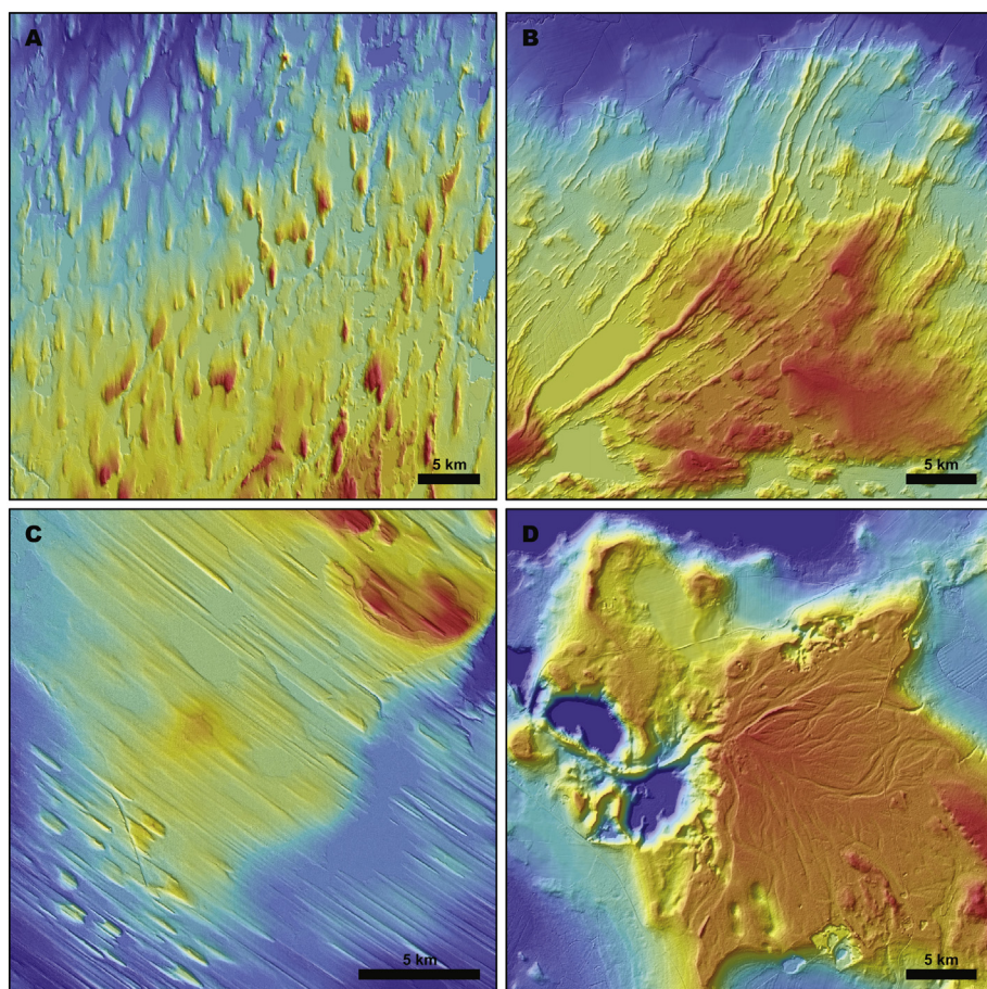
Fig. 9. Examples of landforms in relief-shaded DEMs. Red indicates higher elevations and blue lower elevations. (A) Lineations in N Canada shown in 16 m resolution CDED data. (B) De Geer moraines in SW Finland shown in 2 m resolution LiDAR data. (C) Lineations of the Dubawnt Lake Ice Stream shown in 5 m resolution ArcticDEM mosaic data. (D) Esker-fed ice-contact outwash fan in SW Finland shown in 2 m resolution LiDAR data. See Table 2 for DEM data sources.
