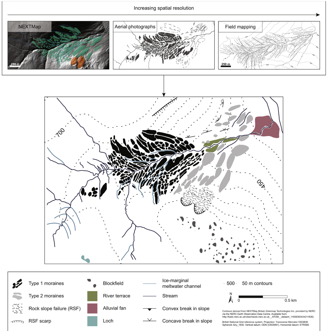
Fig. 14. Geomorphological mapping of Coire Easgainn, Monadhliath, Scotland, using a combination of NEXtMap DSMs, analogue aerial photographs and field mapping. Modified from Boston (2012a, b).
